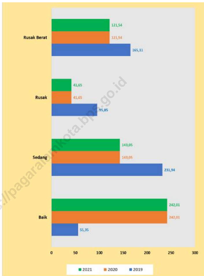
Gambar 8.1 Panjang Jalan Menurut Kondisi Jalan di Kota Pagar Alam (km), 2019–2021 Figures 8.1 Length of Roads by Condition of Roads in Pagar Alam Municipality (km), 2019–2021
