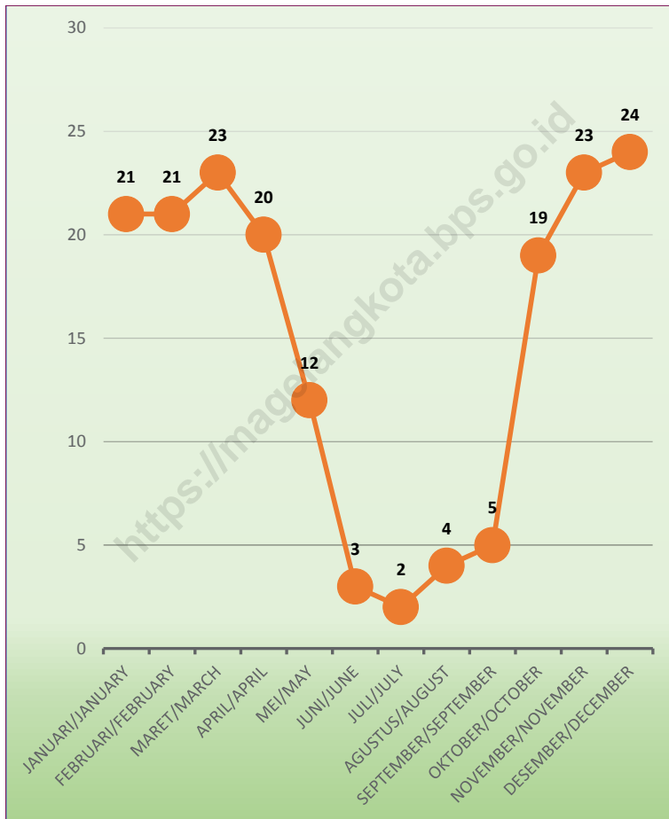
Jumlah Hari Hujan Menurut Bulan di Stasiun CBS 90 Kota Magelang (hari), 2020 Number of Rainy Days By Months at CBS 90 Station in Magelang Municipality (day), 2020
