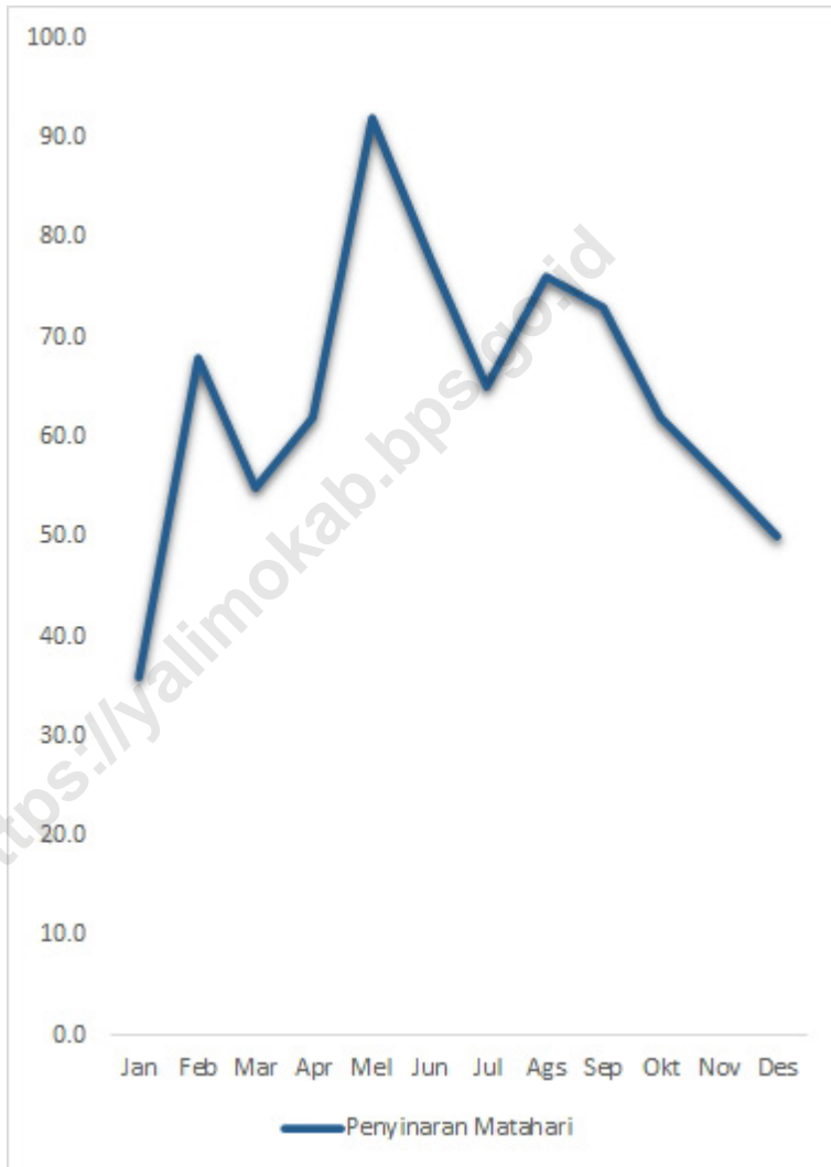
Gambar 1.7 Penyinaran Matahari (%) di Kabupaten Yalimo, 2020 Figures 1.7 Duration of Sunshine (%) of Yalimo Regency, 2020
