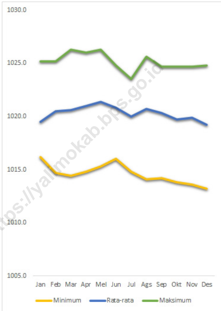
Gambar 1.5 Tekanan Udara (mb) di Kabupaten Yalimo, 2020 Figures 1.5 Atmospheric Pressure (mb) of Yalimo Regency, 2020
