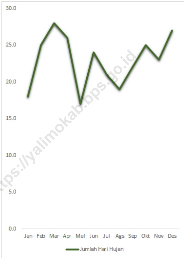
Gambar 1.9 Jumlah Hari Hujan (hari) di Kabupaten Yalimo, 2020 Figures Number of Rainy Days (day) of Yalimo Regency, 2020
