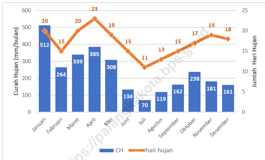
Gambar 2.1 Jumlah Hari Hujan dan Curah Hujan Bulanan Kota Palangka Raya, 2020 Picture Number of Rainy Days and Monthly Rainfall of Palangka Raya Municipality, 2020
