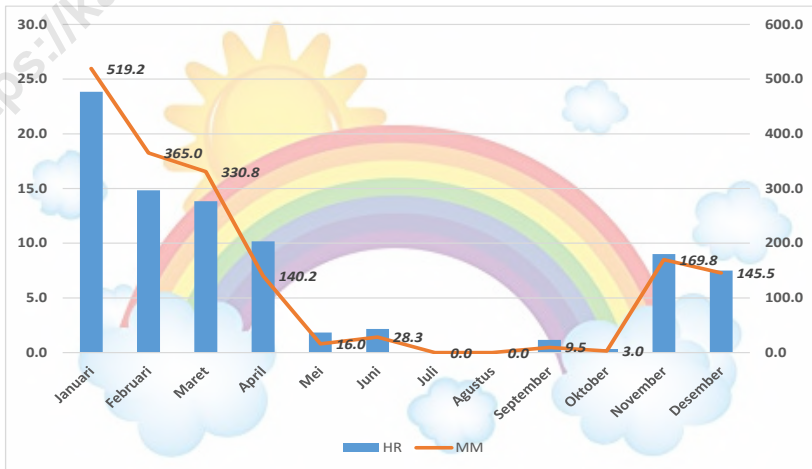
Gambar / Figure 1.3 Hari Hujan dan Curah Hujan Bulanan (mm), 2018 Average Rainfall Day and Rainfall by Month, 2018
