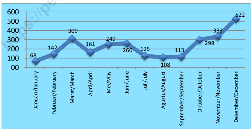
Gambar 2 Jumlah Curah Hujan di Kota Pekanbaru Per Bulan (mm 3 ), 2018 Picture Amount of Precipitation In Pekanbaru Municipality by Month (mm 3 ), 2018
