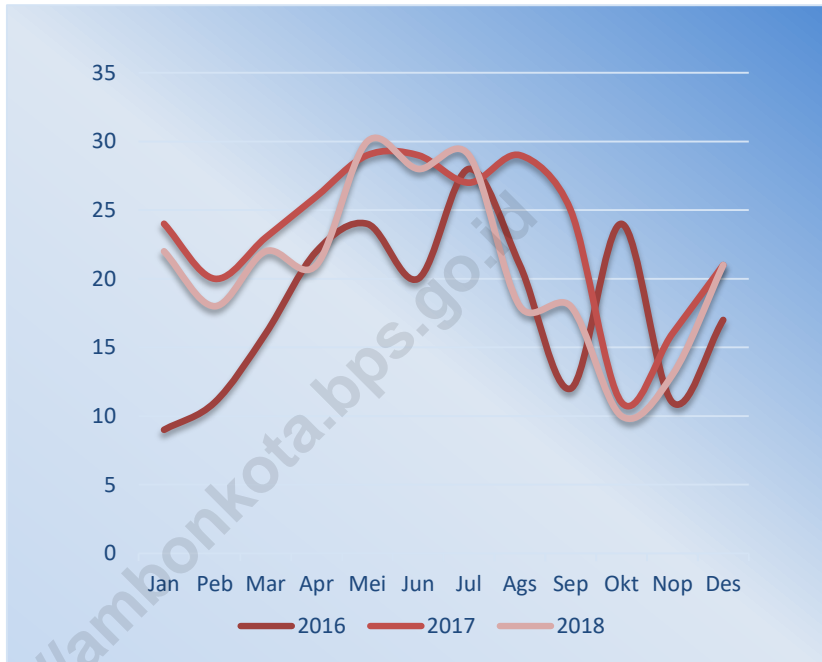
Gambar Jumlah Hari Hujan Menurut Bulan di Kota Ambon, 2016 – 2018 ----- 1 Number Of Rainy Days By Month in Ambon Municipality, Figure 2016 – 2018
