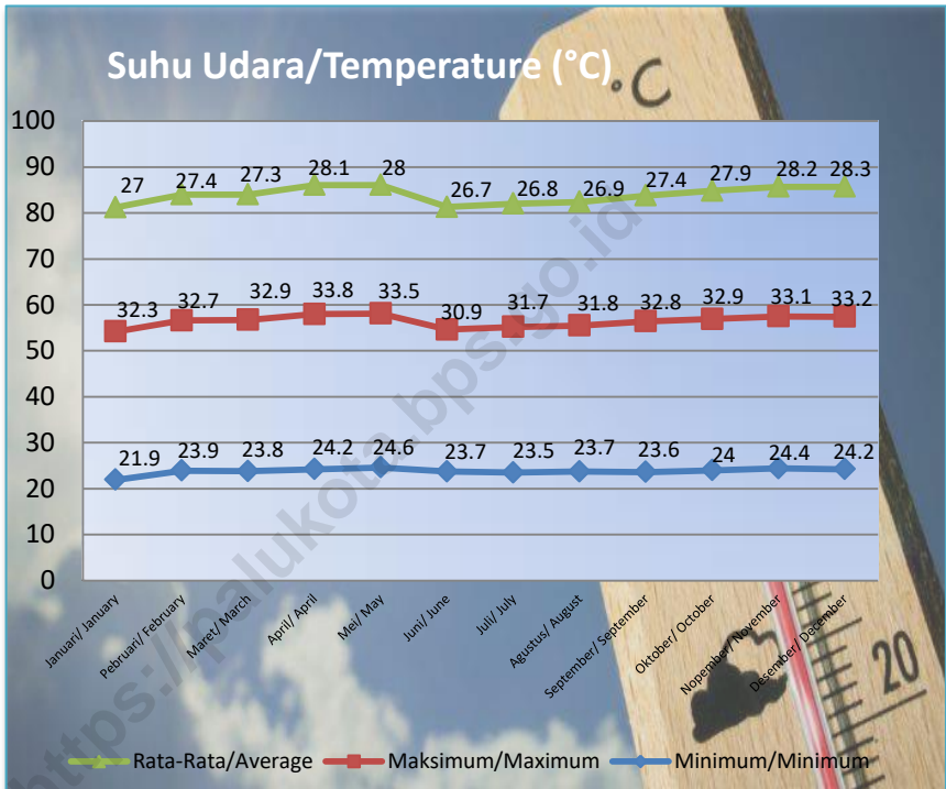
Gambar 2 Suhu Udara Maksimum, Minimum dan Rata-rata Menurut Bulan di Kota Palu, 2017 Picture Maximum, Minimum and Average of Temperature in Palu Municipality by Month, 2017
