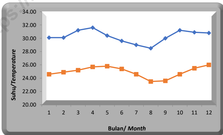
Gambar / Figure : 1.2 Suhu Maksimum dan Minimum di Kabupaten Badung, 2018 (°C) Maximum and Minimum Temperature in Badung Regency, 2018 (°C)
