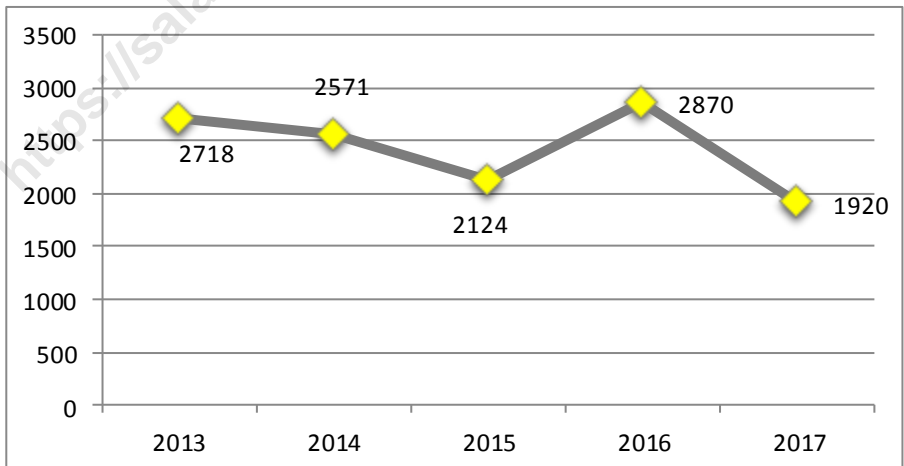
Gambar 1.4 Curah Hujan di Kota Salatiga, 2013 - 2017 (mm) Rainfall in Salatiga Municipality, 2013 - 2017 (mm)
