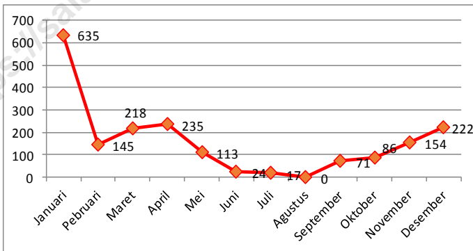
Gambar 1.2 Curah Hujan per Bulan di Kota Salatiga, 2017 (mm) Rainfall per month in Salatiga Municipality, 2017 (mm)
