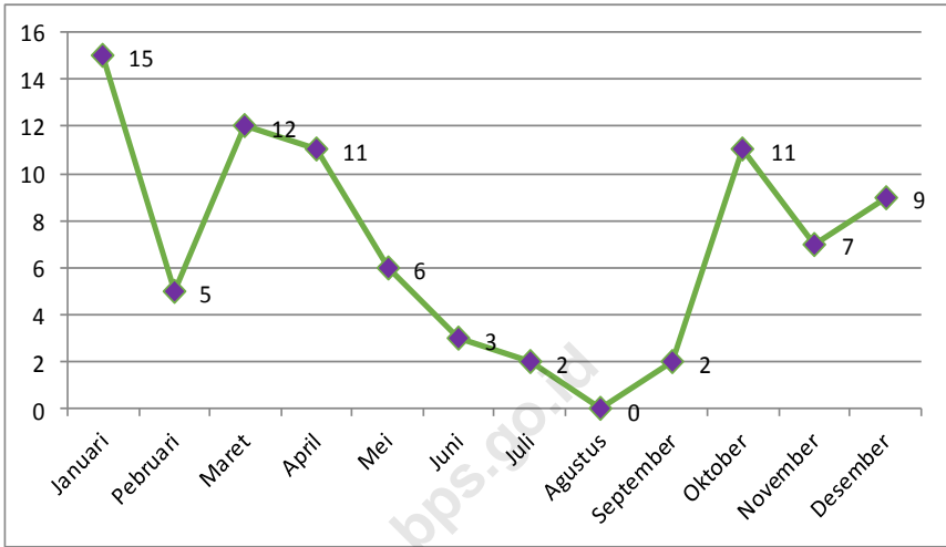
Gambar 1.3 Jumlah Hari Hujan Per Bulan di Kota Salatiga, 2017 (hari) Number of Rainyday per month in Salatiga Municipality, 2017 (days)
