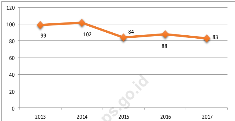
Gambar 1.5 Jumlah Hari Hujan di Kota Salatiga, 2013 - 2017 (hari) Number of Rainyday in Salatiga Municipality, 2013 - 2017 (days)
