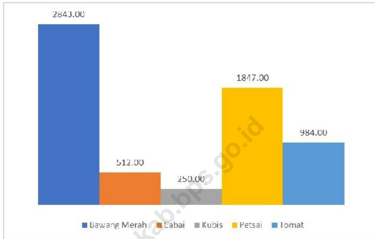
Gambar 5.2 Produksi sayuran dan buah-buahan, 2019 Figures Production of Vegetables and Fruits, 2019
