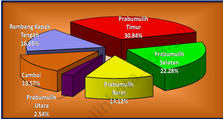
Gambar 1 Luas Wilayah Menurut Kecamatan di Kota Prabumulih (km 2 ), 2017 Picture Total Area by Subdistrict In Prabumulih Municipality (square.km), 2017
