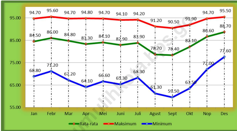
Gambar 3 Kelembaban Udara Maximum, Minimum dan Rata-rata, 2017 Picture The maximum, Minimum and Average Relative Humidity, 2017
