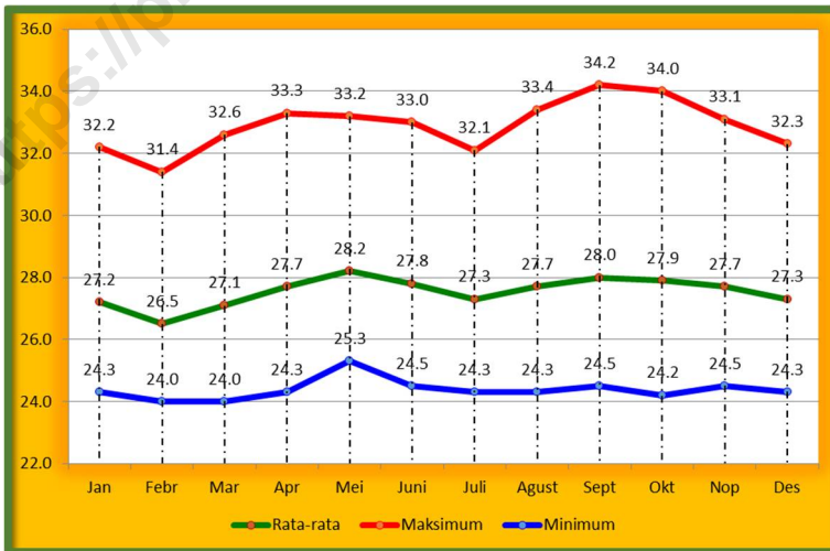
Gambar 2 Suhu Udara Maximum, Minimum dan Rata-rata, 2017 Picture The Maximum, Minimum, and Average Temperature, 2017
