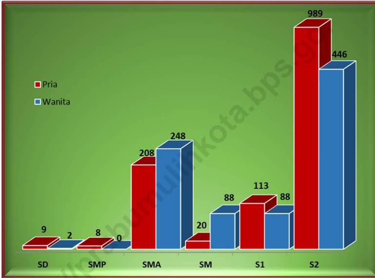
Gambar 4 Jumlah PNS Menurut Pendidikan dan Jenis Kelamin di Kota Prabumulih, 2017 Picture Number of Civil Servant by Education and Sex at Prabumulih Municipality, 2017
