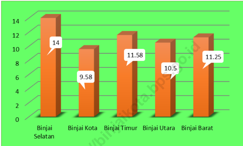
Gambar 1.2 Perbandingan Curah Hujan Menurut Kecamatan di Kota Binjai, (hari) 2019 Picture Comparison of Precipitations by Sub District in Binjai Municipality, (days) 2019
