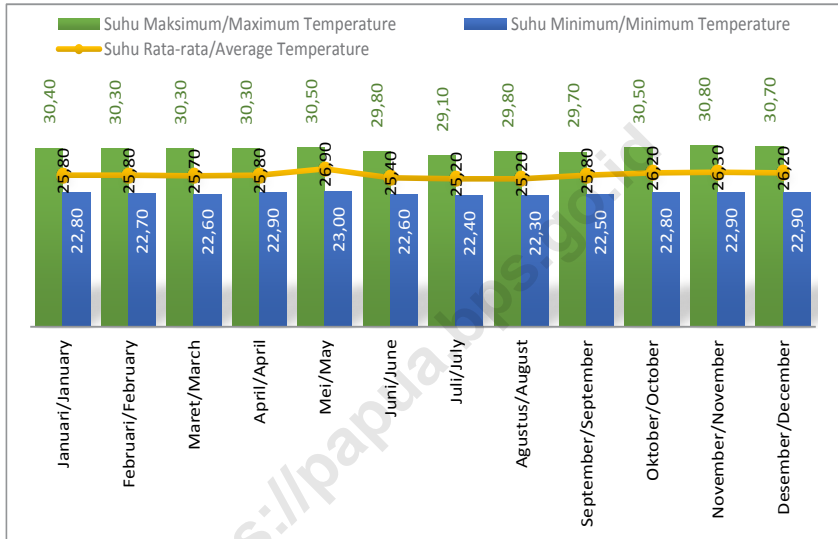
Gambar 1.11. Rata-rata Suhu Udara Menurut Bulan Pengamatan di Provinsi Papua (°C), 2017 Picture Average of Temperature by Observation Month in Papua Province (°C), 2017
