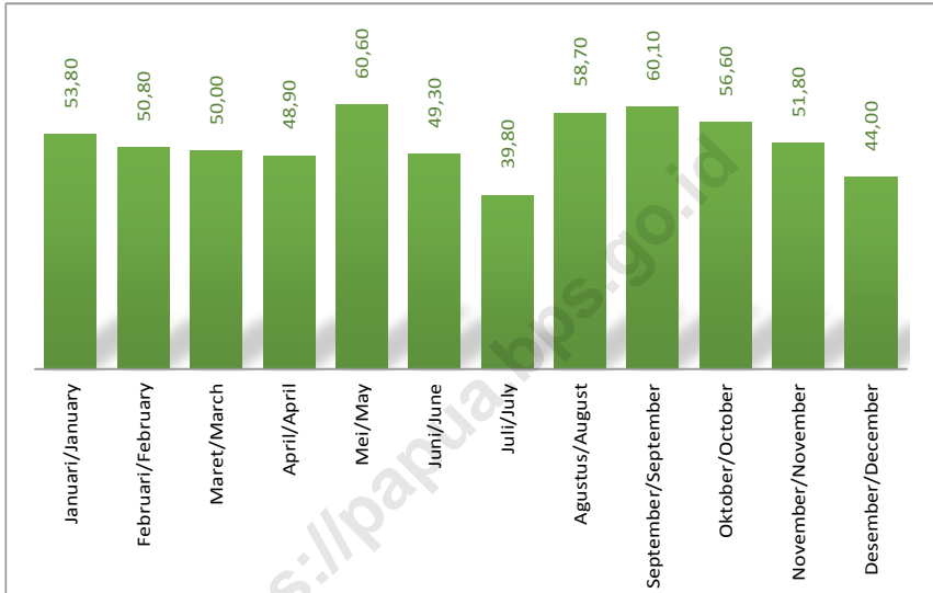
Gambar 1.15. Rata-rata Penyinaran Matahari Menurut Bulan Pengamatan di Provinsi Papua (persen), 2017 Average of Duration of Sunshine by Observation Month in Papua Province (percent), 2017
