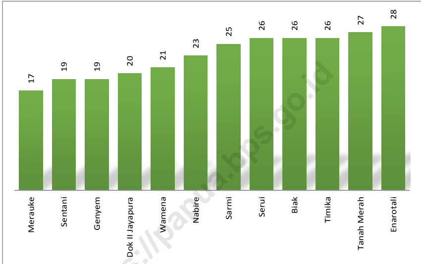
Gambar 1.9. Rata-rata Hari Hujan Menurut Stasiun Pengamatan di Provinsi Papua (hari), 2017 Average of Raining Days by Observation Station in Papua Province (days), 2017
