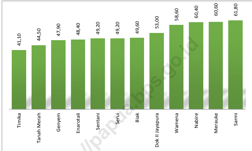
Gambar 1.10. Rata-rata Penyinaran Matahari Menurut Stasiun Pengamatan di Provinsi Papua (persen), 2017 Average of Duration of Sunshine by Observation Station in Papua Province (percent), 2017
