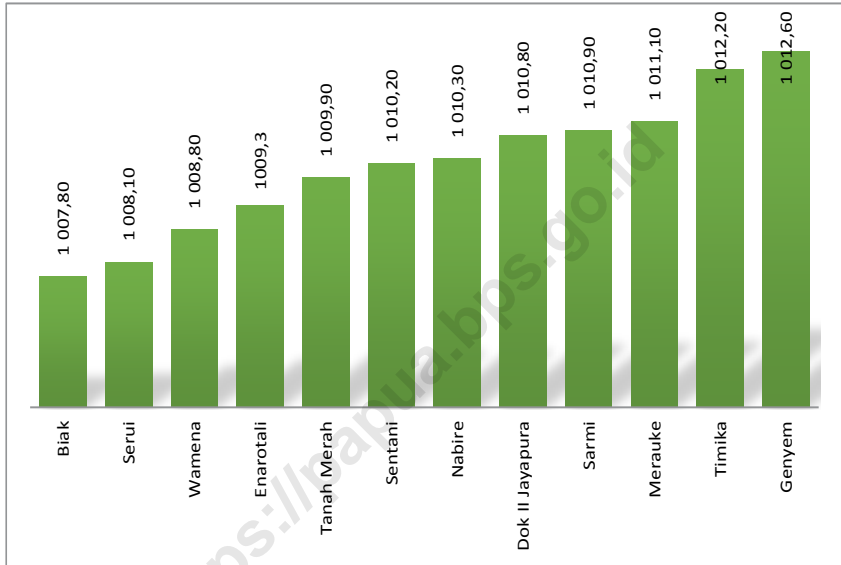
Gambar 1.6. Rata-rata Tekanan Udara Menurut Stasiun Pengamatan di Provinsi Papua (mb), 2017 Average of Atmospheric Pressure by Observation Station in Papua Province (mb), 2017
