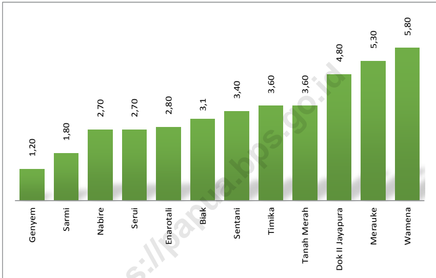
Gambar 1.7. Rata-rata Kecepatan Angin Menurut Stasiun Pengamatan di Provinsi Papua (knot), 2017 Picture Average of Wind Velocity by Observation Station in Papua Province (knot), 2017
