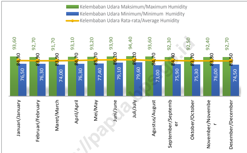
Gambar 1.12. Rata-rata Kelembaban Udara Menurut Bulan Pengamatan di Provinsi Papua (persen), 2017 Picture Average of Humidity by Observation Month in Papua Province (percent), 2017
