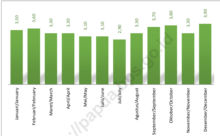
Gambar 1.14. Rata-rata Kecepatan Angin Menurut Bulan Pengamatan di Provinsi Papua (knot), 2017 Average of Wind Velocity by Observation Month in Papua Province (knot), 2017
